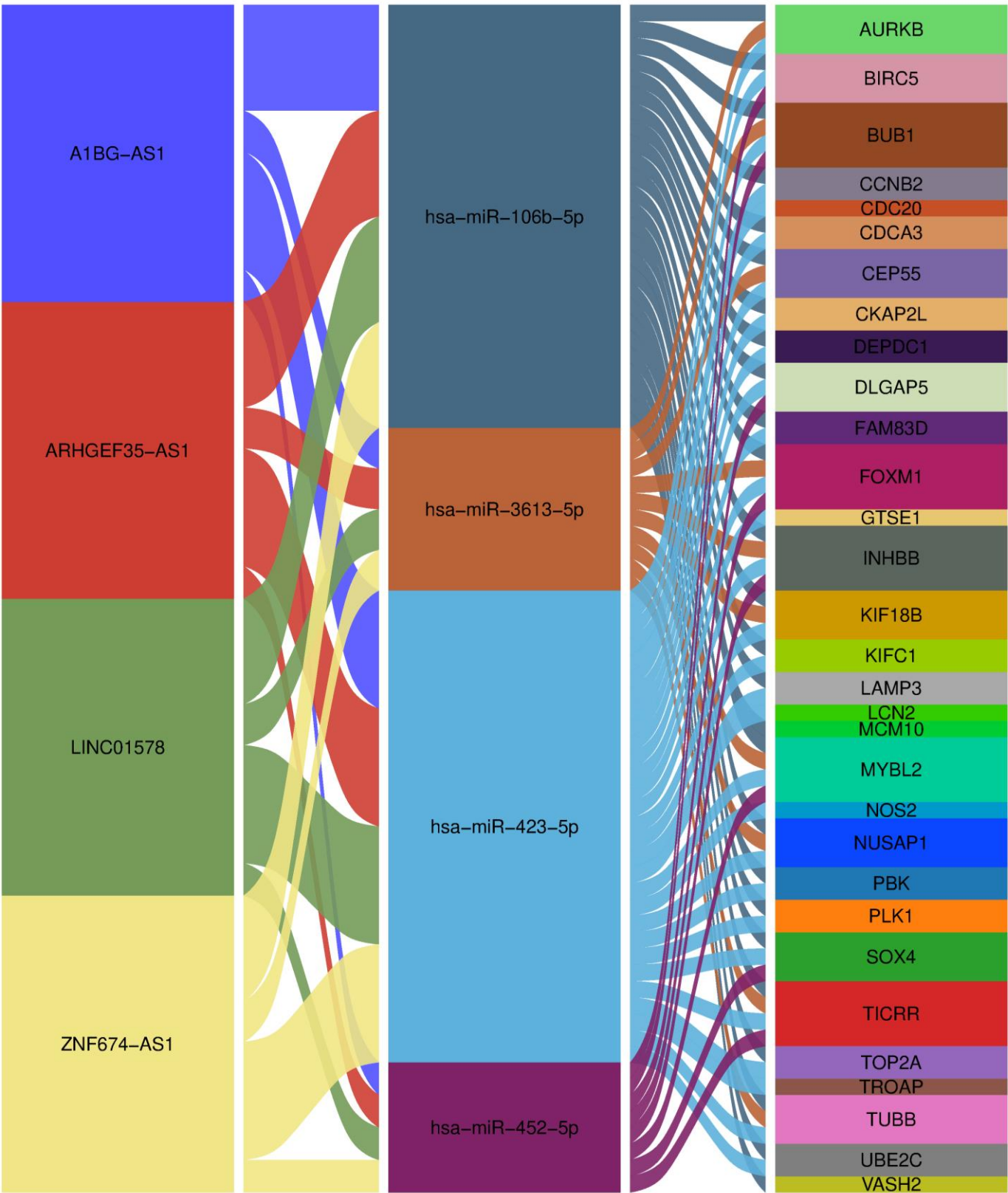
Figure5. The Core ceRNA Network in POI. The competing endogenous RNA (ceRNA) network integrating 4 lncRNAs , 4 miRNAs , and 31 mRNAs . This network posits that exosome-derived lncRNAs regulate mRNA expression by sponging miRNAs, revealing a potential central regulatory axis in POI pathogenesis.
